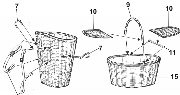
Metal parts
